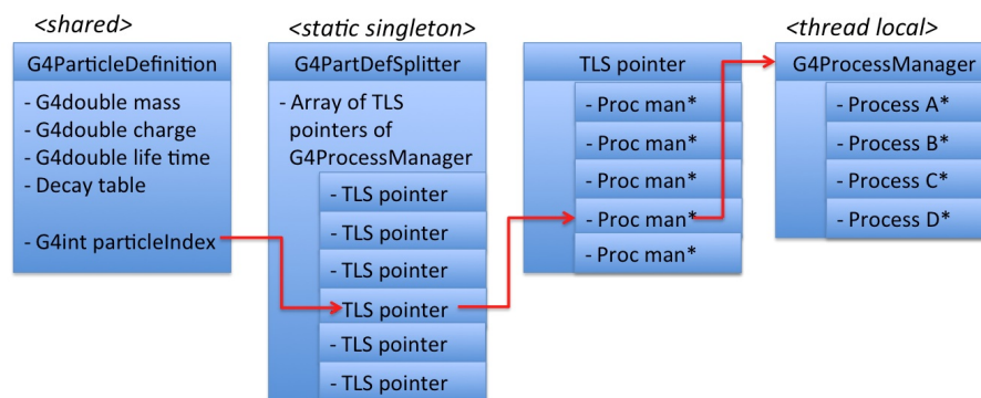
Fig. 2.30: Simplified view of the split-class mechanism
