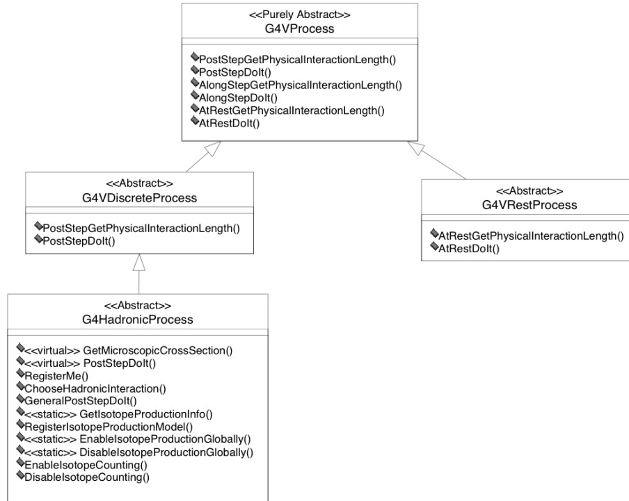
Fig. 3.3: Level 1 implementation framework of the hadronic category of GEANT4.
